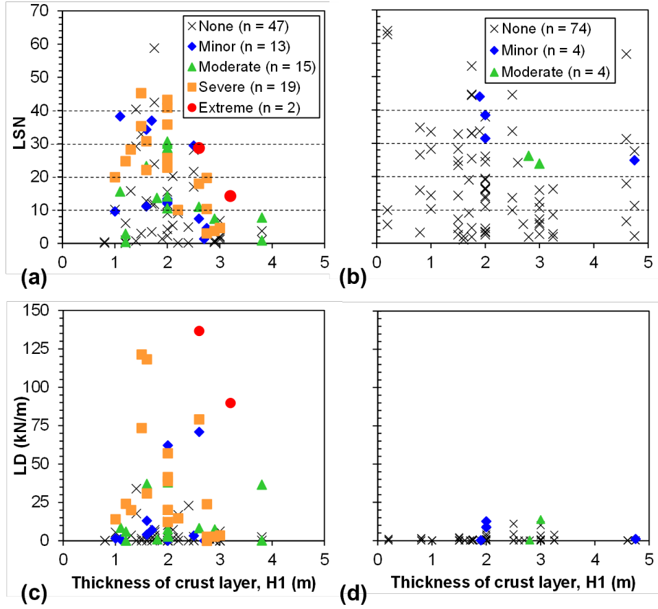
Figure 3.4. Distribution of liquefaction ejecta demand parameters vs. crust thickness for field case histories (from Hutabarat and Bray 2022)
