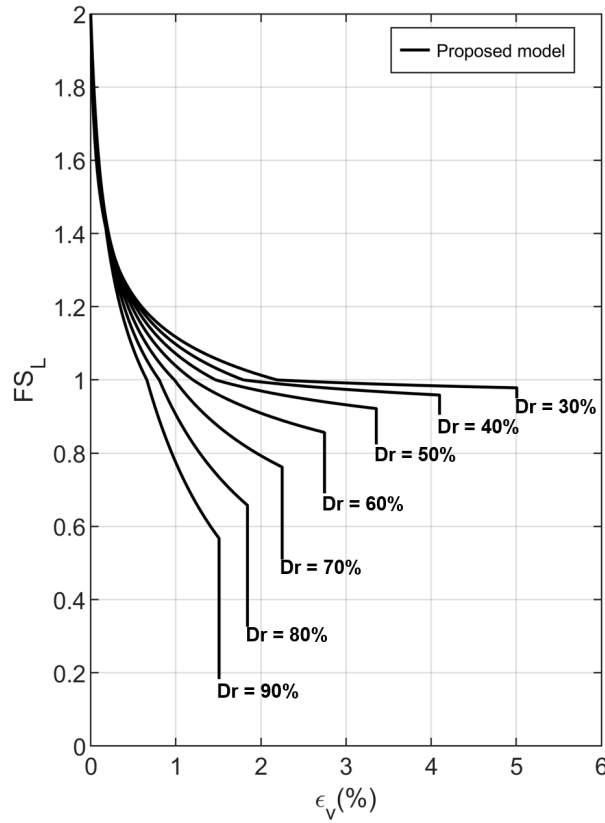
Figure 5.5. Relationship between \varepsilon_v and FS_L in terms of D_r (Olaya and Bray 2022b)
